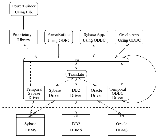
Figure 4. Using ODBC as the Stratum
