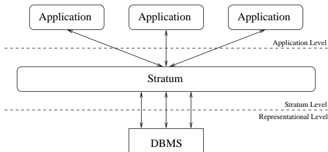
Figure 1. The Stratum Approach
