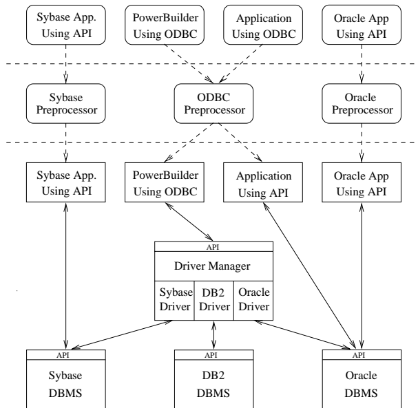
Figure 6. The Preprocessor Architecture
