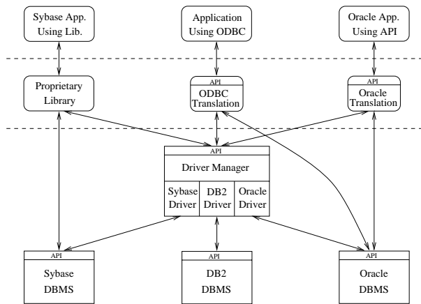
Figure 2. Interposing a Stratum Directly
