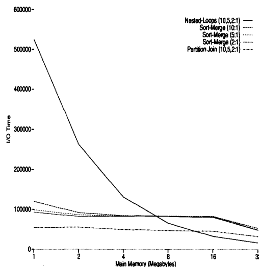
Figure 6: Performance Effects of Main Memory
