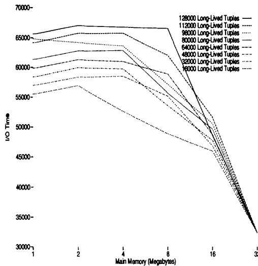
Figure 8: Relative Effects of Main Memory Size and Tuple Caching
