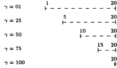
Figure 8: Shrink\_s(\gamma, ([1, 20], Uniform)) for several values of \gamma
