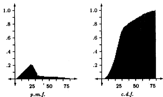
Figure 2: A "probably early" distribution
